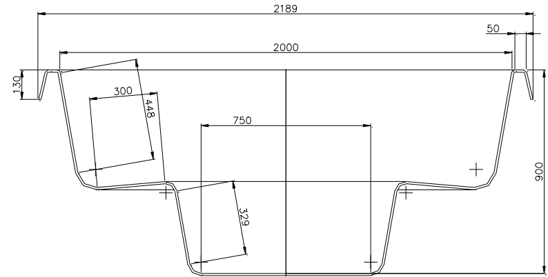
SECTION C-C
