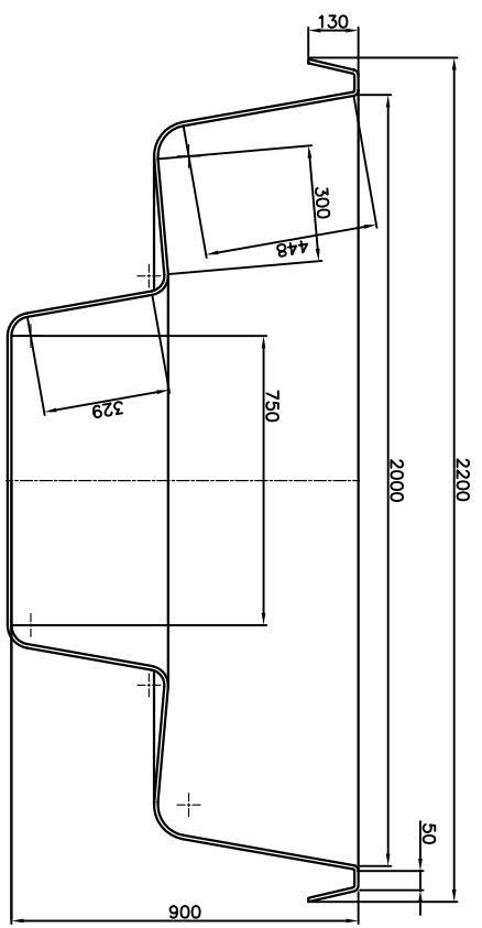
SECTION C-C
